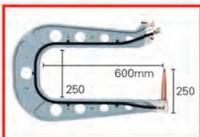
Insulated C9 (CEL020078)
