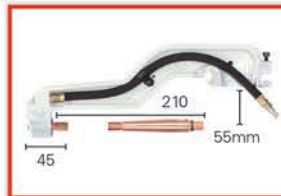
C2 Arm (CEL019133) Insulated C2 (CEL022386)
